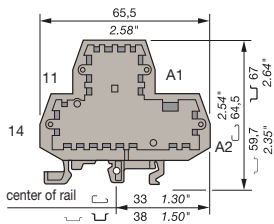
M 4/9.R111...
