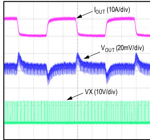
TRANSIENT RESPONSE
