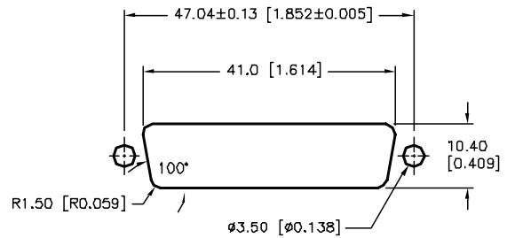
Panel Cutout
