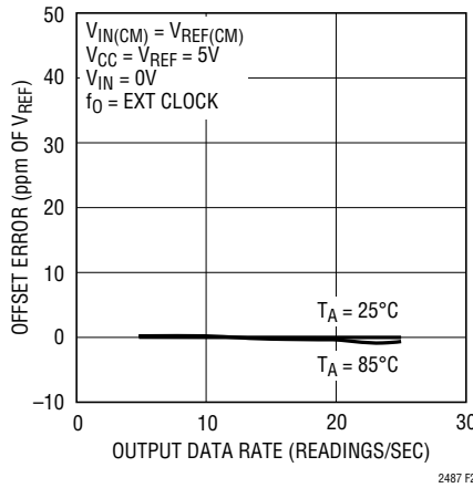
Figure 29. Offset Error vs Output Data Rate and Temperature
