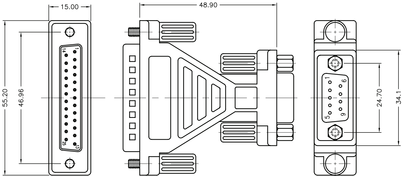
DB-25 Pin Male
