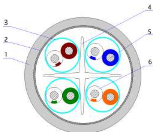
Cross Section
