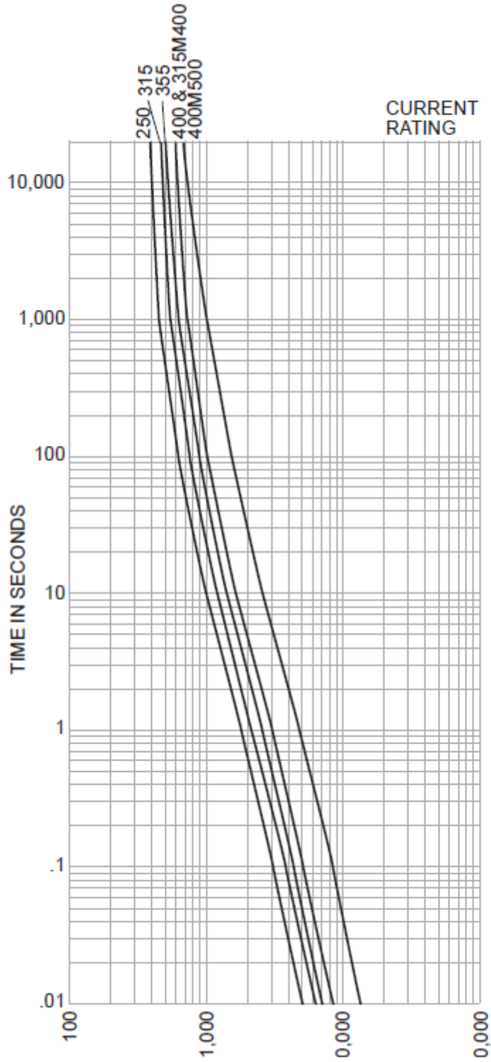
Time-Current Characteristic Curve (Full Size Curves Available)
