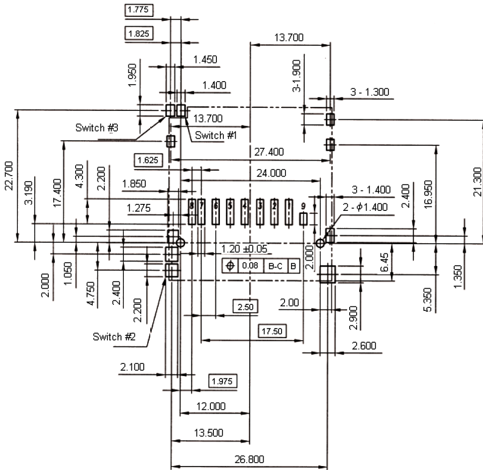
SD Card PIN Assignment
