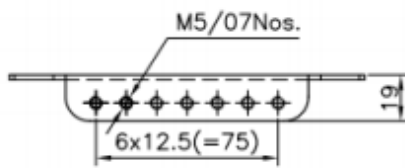
DETAIL OF MOUNTING RAIL
