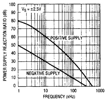
LT1218 Power Supply Rejection Ratio vs Frequency
