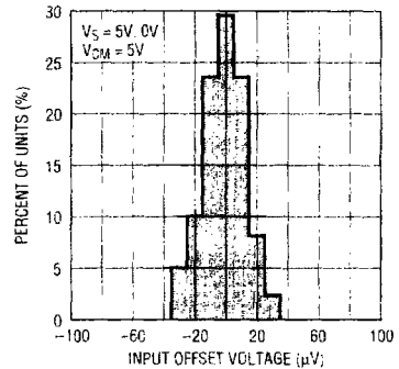
V_{OS} Distribution, V_{CM} = 5V
