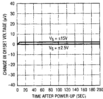
Input Offset Drift vs Time
