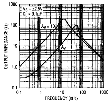
LT1219 Closed Loop Output Impedance vs Frequency
