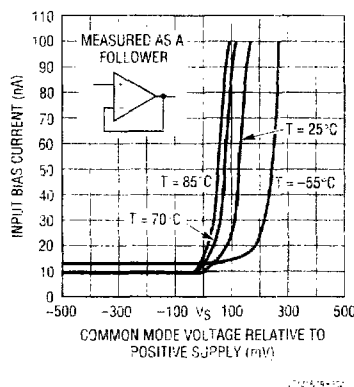
Figure 2. Input Bias Current vs Common Mode Voltage
