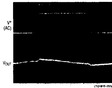
Figure 7b. LT1219 Power Supply Rejection Test
