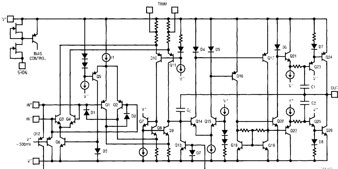
Figure 1. LT1218 Simplified Schematic Diagram
