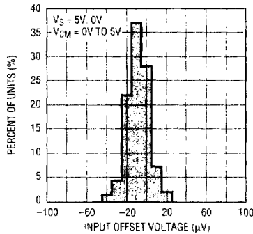
V_{OS} Shift, V_{CM} = 0V to 5V
