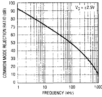
LT1218 Common Mode Rejection Ratio vs Frequency
