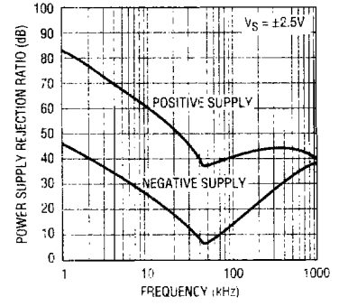
LT1219 Power Supply Rejection Ratio vs Frequency
