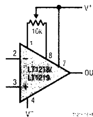
Figure 6. Optional Offset Nulling
