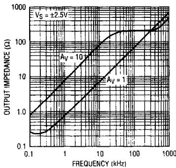
LT1218 Closed Loop Output Impedance vs Frequency
