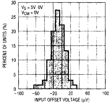
V_{OS} Distribution, V_{CM} = 0V
