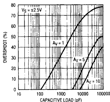
LT1218 Capacitive Load Handling
