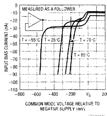
Figure 3. Input Bias Current vs Common Mode Voltage
