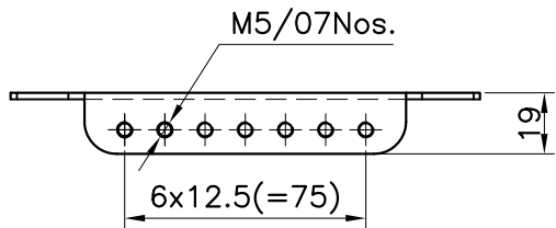
DETAIL OF MOUNTING RAIL
