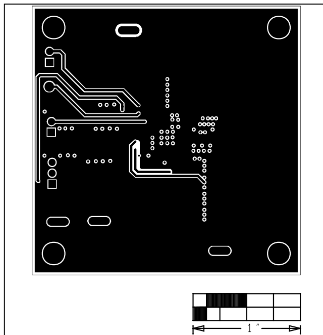
Figure 5. MAXM17504 EV Kit PCB Layout—PGND Layer 3
