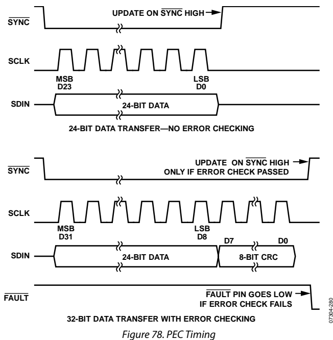
Figure 78. PEC Timing
