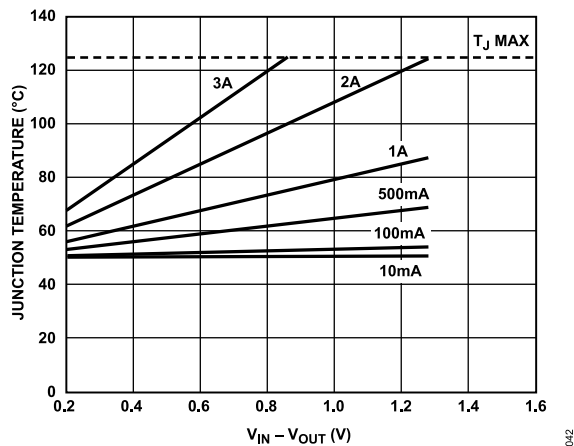
Figure 44. 1000 mm 2 of PCB Copper, T B = 50°C, LFCSP
