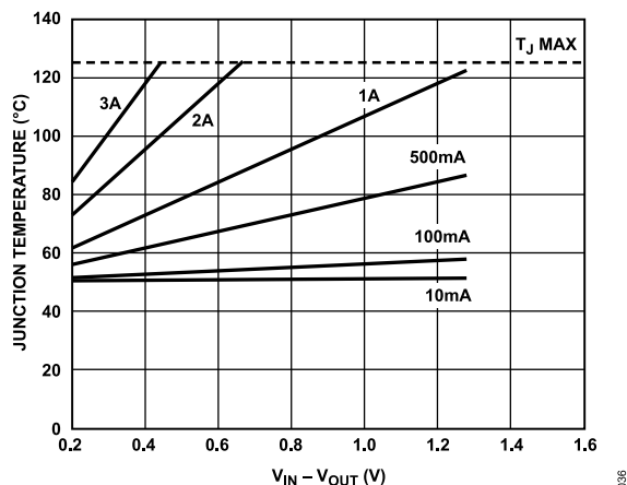
Figure 38. 6400 mm 2 of PCB Copper, T A = 50°C
