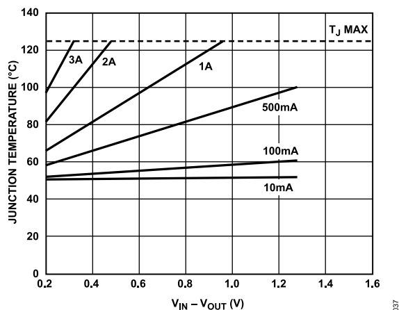
Figure 39. 500 mm 2 of PCB Copper, T A = 50°C
