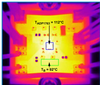
Figure 45. Thermal Image of the ADP1763 Evaluation Board at I LOAD = 3 A, V IN = 1.5 V, V OUT = 1.3 V, T B = 92°C
