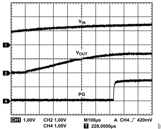
Figure 29. Typical PG Behavior vs. V_{OUT} , V_{IN} Rising ( V_{OUT} = 1.3\text{ V} )
