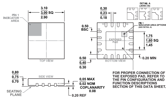
Figure 49. 16-Lead Lead Frame Chip Scale Package [LFCS] 3 mm x 3 mm Body and 0.75 mm Package Height (CP-16-22) Dimensions shown in millimeters
