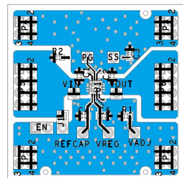
Figure 47. Typical Board Layout, Top Side
