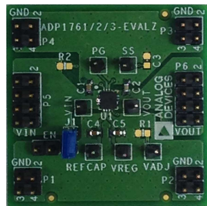
Figure 46. Evaluation Board
