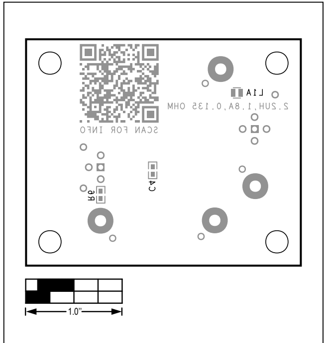
MAX38641A WLP EV Kit—Bottom Silkscreen
