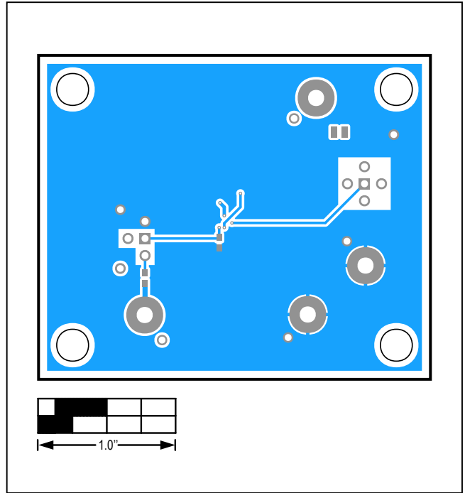
MAX38641A WLP EV Kit—Bottom View
