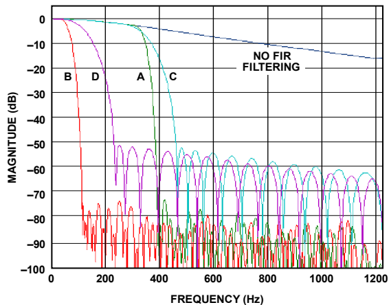
Figure 50. FIR Filter Frequency Response Curves
