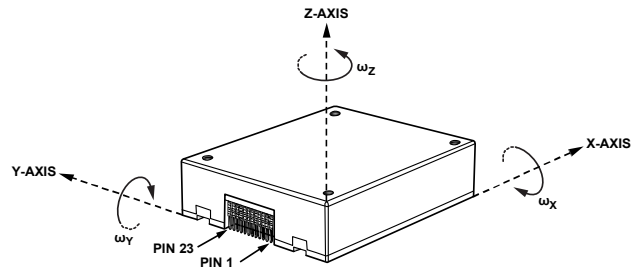
Figure 38. Gyroscope Axis and Polarity Assignments
