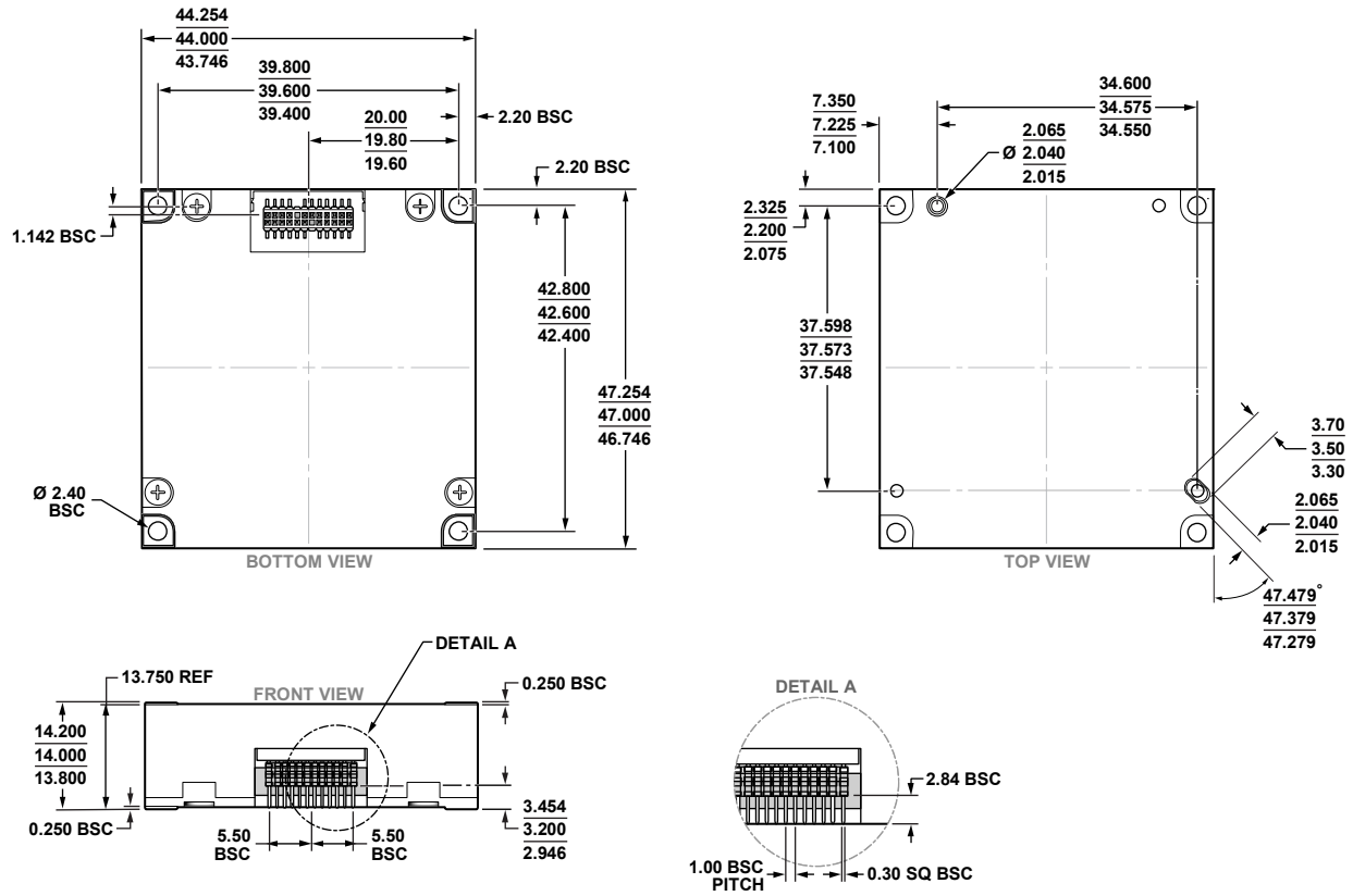
Figure 54. 24-Lead Module with Connector Interface [MODULE] (ML-24-9) Dimensions shown in millimeters
