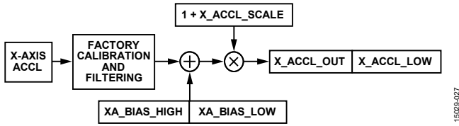
Figure 47. User Calibration Signal Path, Accelerometers
