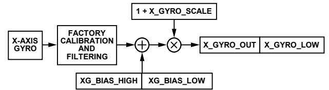
Figure 46. User Calibration Signal Path, Gyroscopes
