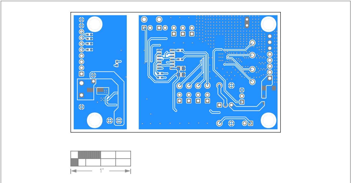
MAX14919A EV Kit PCB Layout—Bottom View
