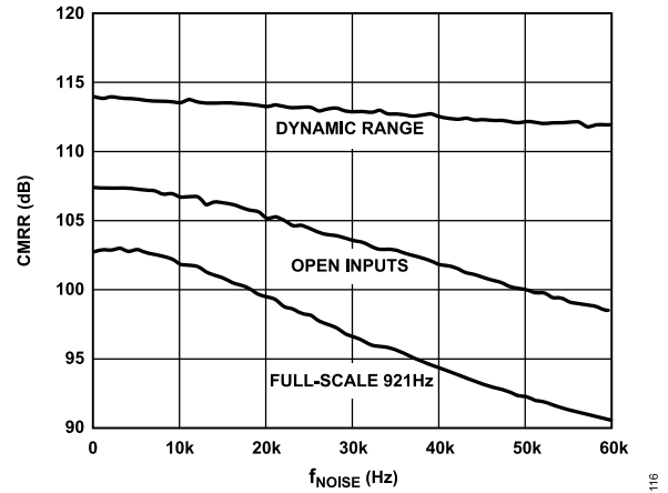
Figure 22. AD7766 CMRR vs. Common-Mode Ripple Frequency ( f_{noise} )
