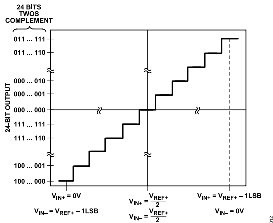
Figure 28. AD7766/AD7766-1/AD7766-2 Transfer Function
