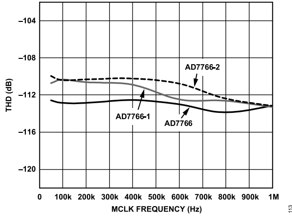
Figure 19. AD7766/AD7766-1/AD7766-2 THD vs. MCLK Frequency
