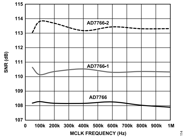
Figure 20. AD7766/AD7766-1/AD7766-2 SNR vs. MCLK Frequency
