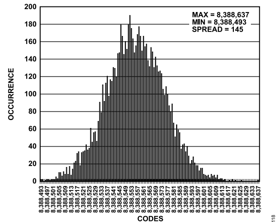
Figure 23. AD7766 24-Bit Histogram
