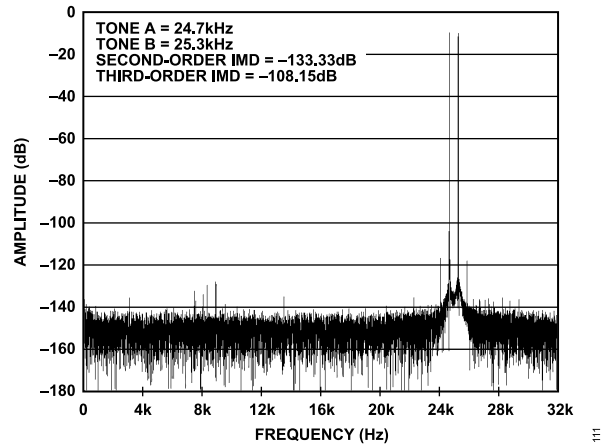
Figure 17. AD7766-1 IMD FFT, 25 kHz Center Frequency
