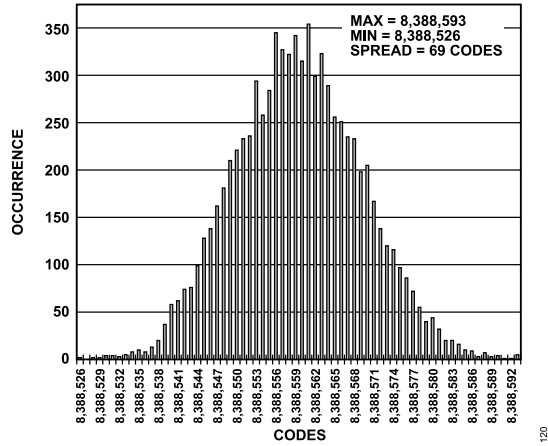
Figure 25. AD7766-2 24-Bit Histogram
