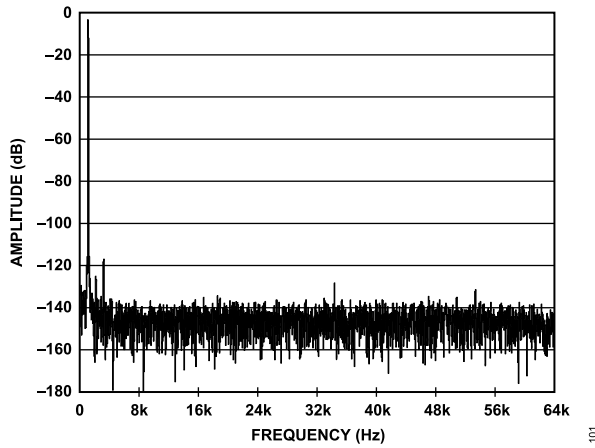
Figure 7. AD7766 FFT, 1 kHz, -0.5 dB Input Tone
