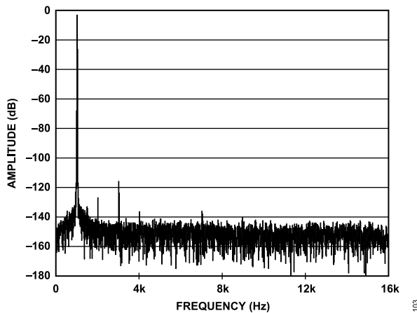
Figure 9. AD7766-2 FFT, 1 kHz, -0.5 dB Input Tone
