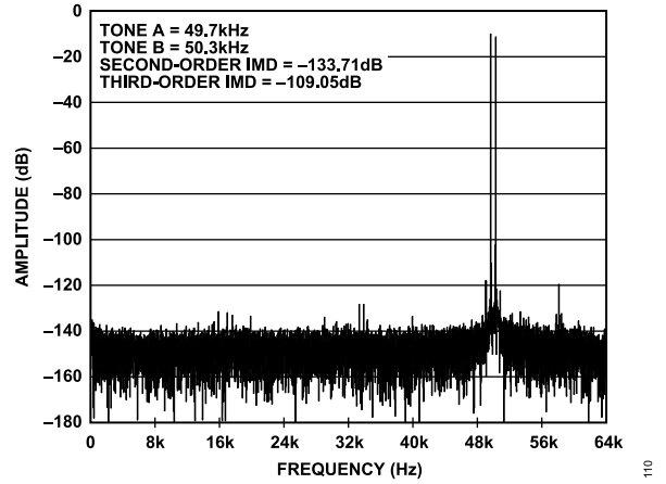
Figure 16. AD7766 IMD FFT, 50 kHz Center Frequency
