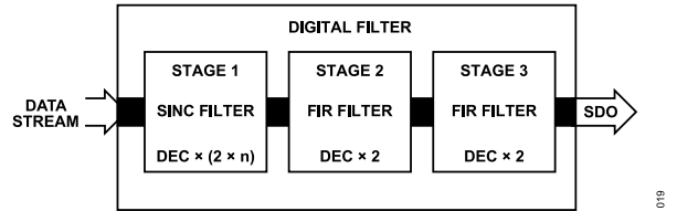
Figure 31. FIR Filter Stages ( n = 1 for AD7766, n = 2 for AD7766-1, n = 4 for AD7766-2)
