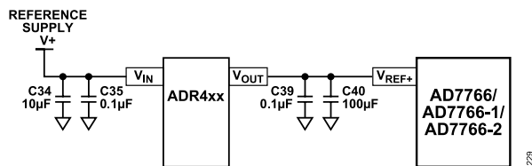
Figure 46. AD7766/AD7766-1/AD7766-2 Reference Input Configuration
