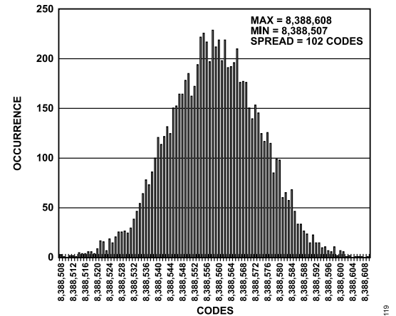
Figure 24. AD7766-1 24-Bit Histogram
