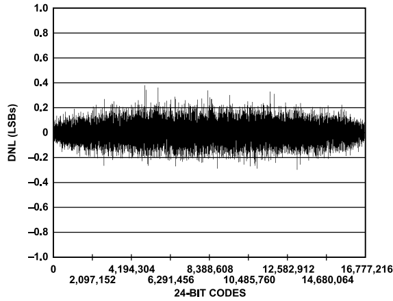
Figure 26. AD7766/AD7766-1/AD7766-2 24-Bit DNL
