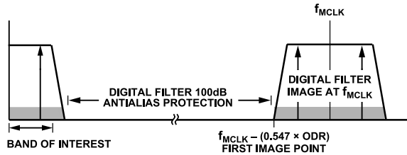
Figure 42. AD7766/AD7766-1/AD7766-2 Spectrum
