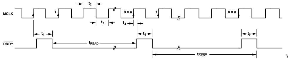
Figure 2. \overline{DRDY} vs. MCLK Timing Diagram, n = 1 for AD7766 (Decimate by 8), n = 2 for AD7766-1 (Decimate by 16), n = 4 for AD7766-2 (Decimate by 32)
