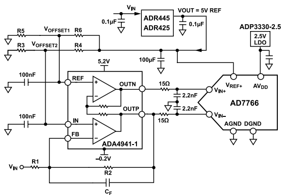
Figure 41. Driving the AD7766 from a Single-Ended Source
