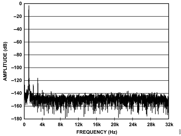
Figure 8. AD7766-1 FFT, 1 kHz, -0.5 dB Input Tone
