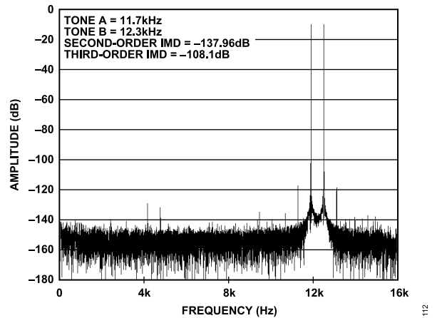
Figure 18. AD7766-2 IMD FFT, 12 kHz Center Frequency
