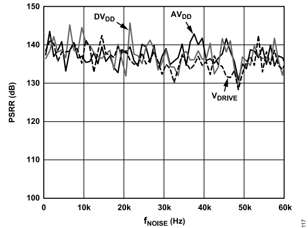
Figure 21. AD7766 Power Supply Sensitivity vs. Supply Ripple Frequency ( f_{noise} ) with Decoupling Capacitors
