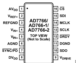
Figure 6. 16-Lead TSSOP Pin Configuration
