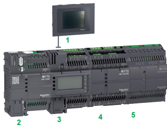
1 Color touch screen display 2 Secure Interface (Plug-in version) 3 M172 Optimized logic controller 4 I/O expansion module 5 Electronic expansion valve driver
