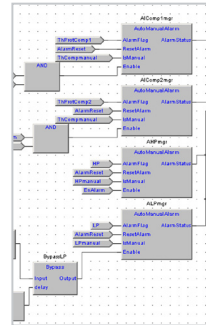
Function Block Diagram language (FBD)
