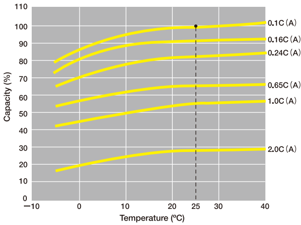
● MSE Series Temperature-Capacity Characteristics
