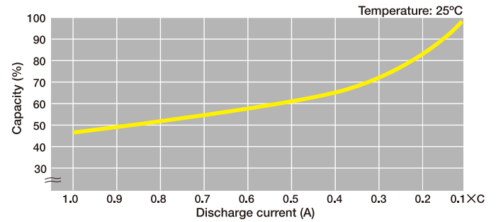
● HSE Series Discharge Current-Capacity Characteristics
