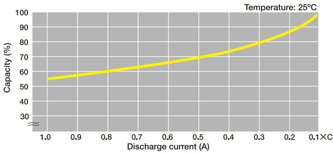
● MSE Series Discharge Current-Capacity Characteristics
