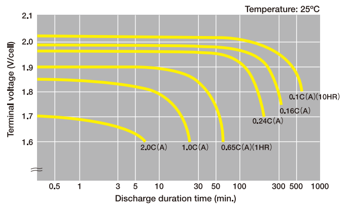
● HSE Series Discharge Characteristics with Varying Discharge Rate
