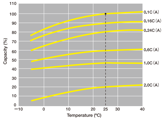
● HSE Series Temperature-Capacity Characteristics
