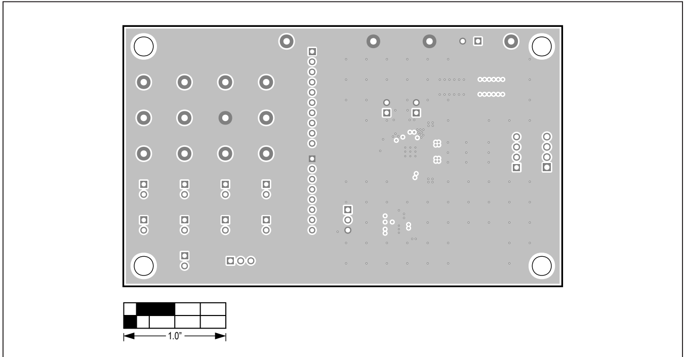
MAX22211 EV Kit—Layer 2
