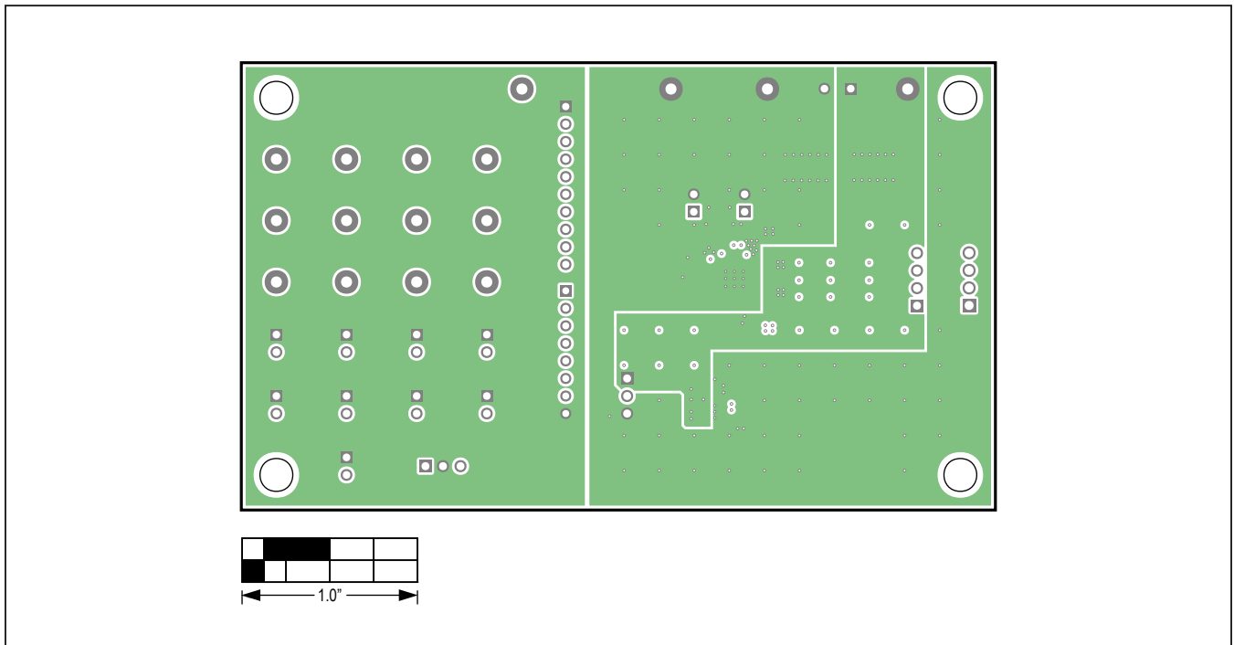
MAX22211 EV Kit—Layer 3
