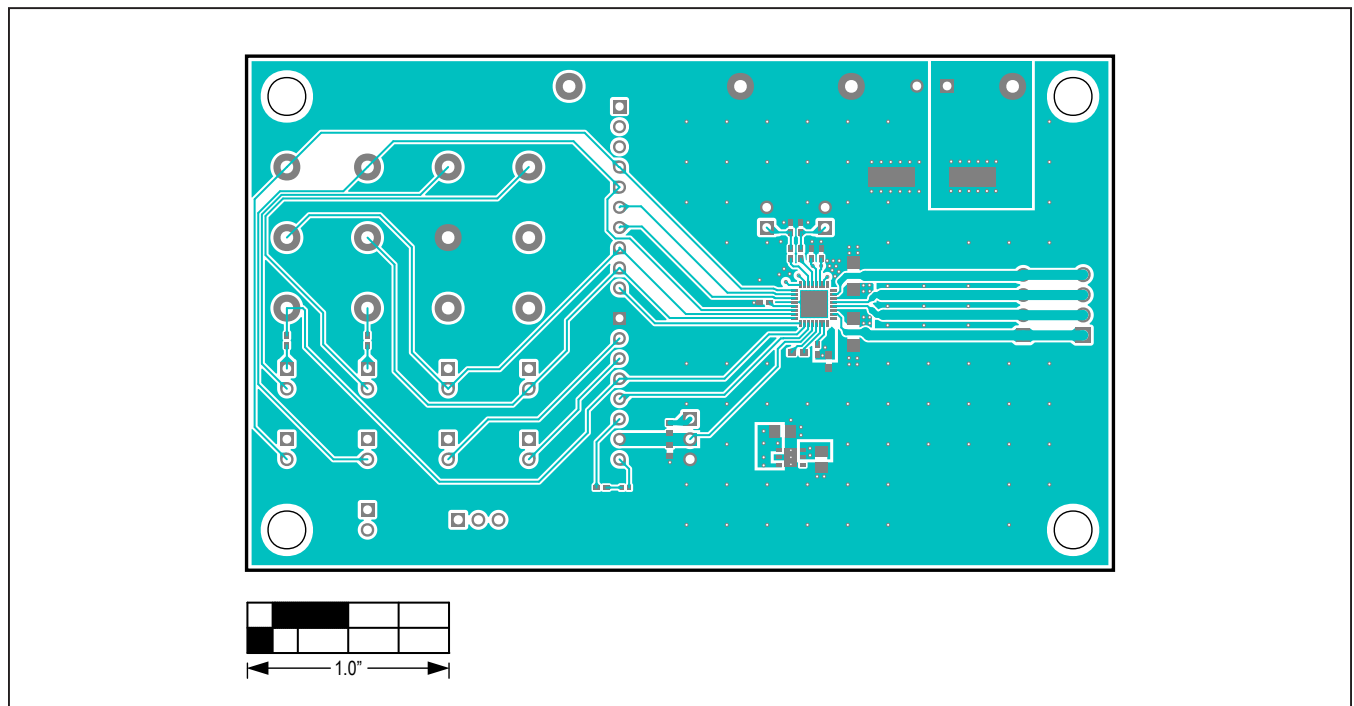
MAX22211 EV Kit—Top Layer
