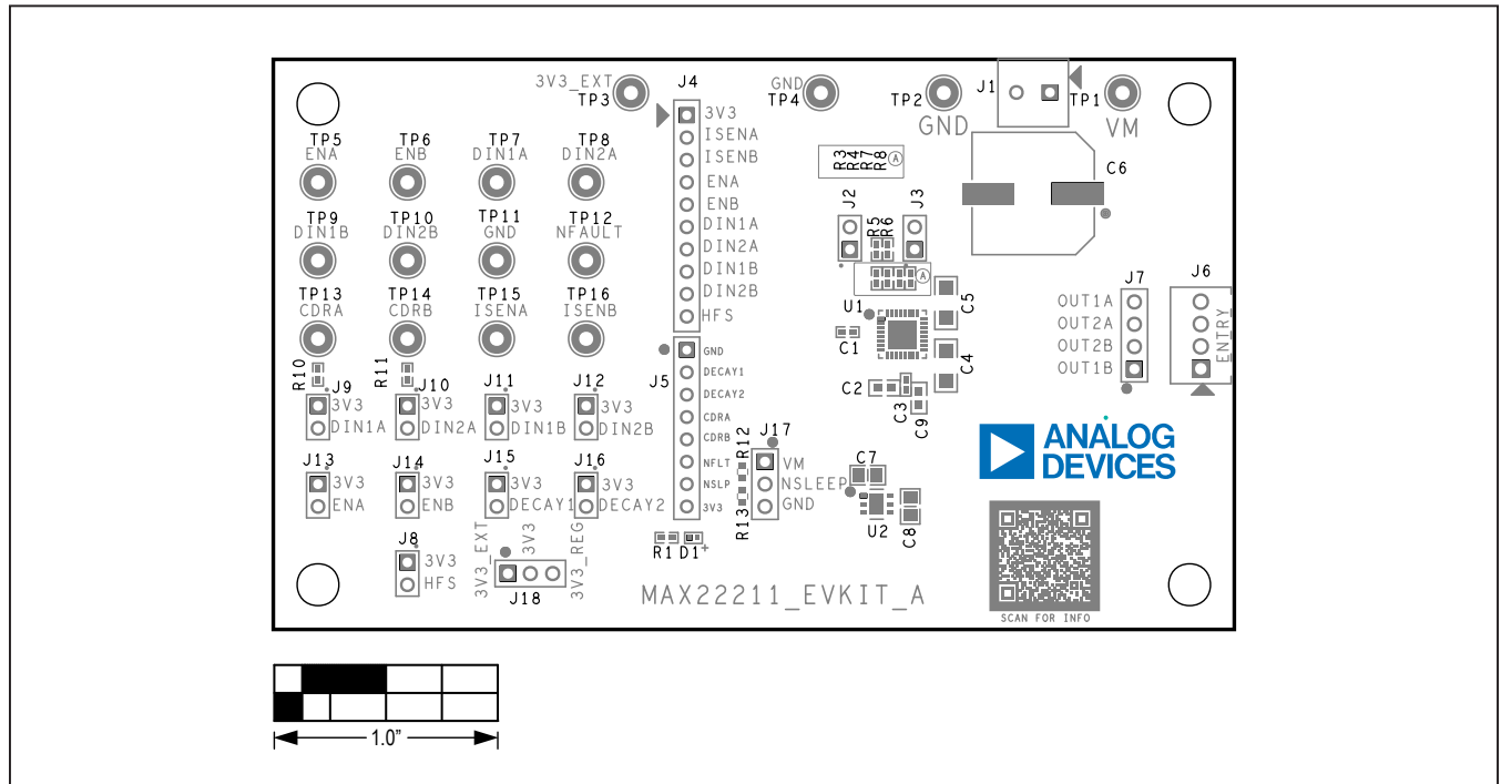
MAX22211 EV Kit—Silkscreen Top Layer
