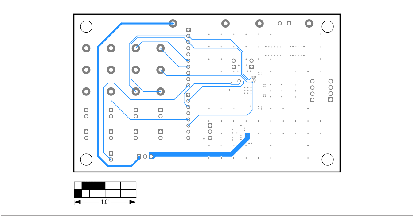
MAX22211 EV Kit—Bottom Layer
