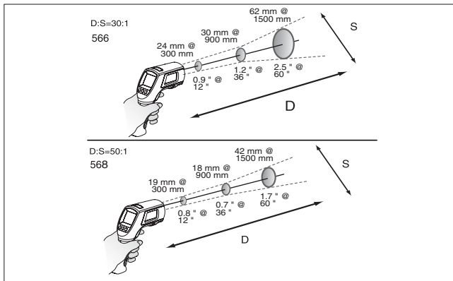
Figure 5. Distance and Spot Size
