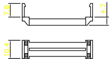
Strain Relief
