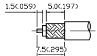
STRIPPING DIMENSION
