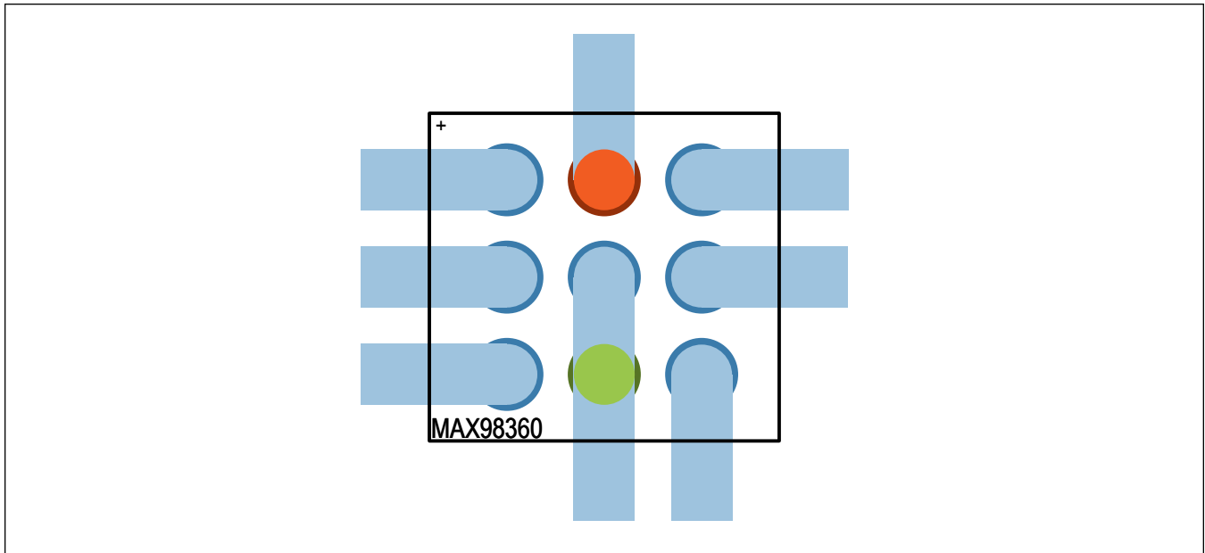
Figure 16. GAIN_SLOT Tied to GND (Gain is 12dB in I 2 S and Left-Justified Modes)
