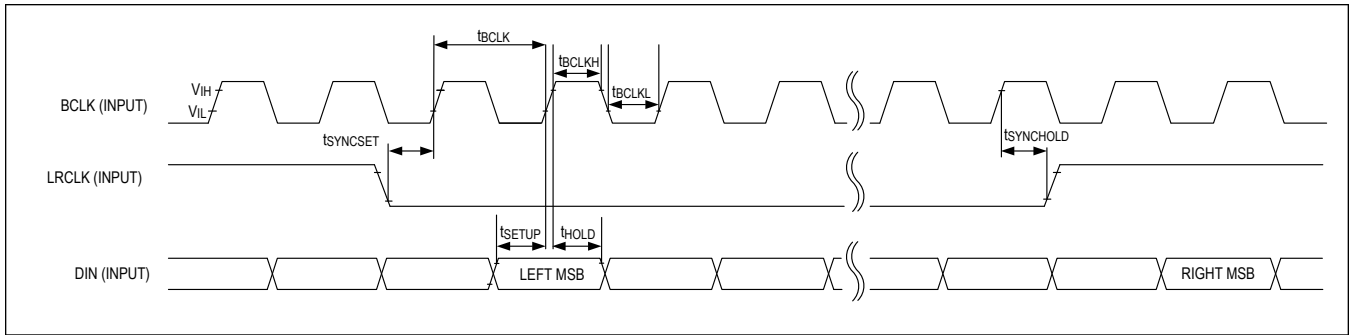
Figure 6. I 2 S Timing Diagram (MAX98360A and MAX98360C)
