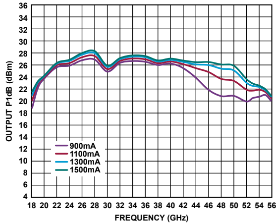
Figure 59. Output P1dB vs. Frequency for Various Supply Currents, V_{DD} = 3\text{ V}
