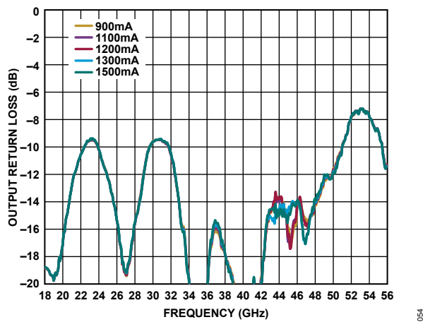
Figure 55. Output Return Loss vs. Frequency for Various Supply Currents, V_{DD} = 3\text{ V}
