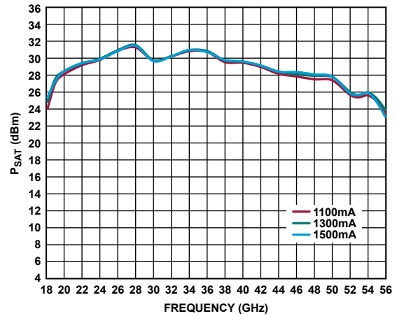
Figure 63. P_{SAT} vs. Frequency for Various Supply Currents, V_{DD} = 4\text{ V}
