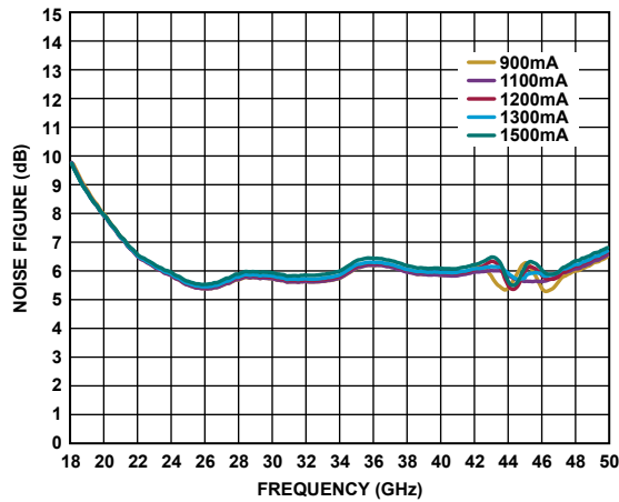
Figure 61. Noise Figure vs. Frequency for Various Supply Currents, V_{DD} = 3\text{ V}
