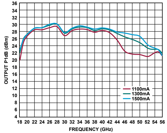
Figure 62. Output P1dB vs. Frequency for Various Supply Currents, V_{DD} = 4\text{ V}
