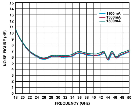
Figure 64. Noise Figure vs. Frequency for Various Supply Currents, V_{DD} = 4\text{ V}
