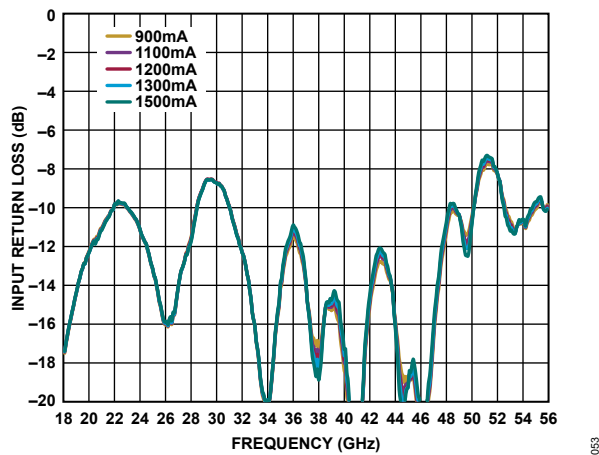
Figure 54. Input Return Loss vs. Frequency for Various Supply Currents, V_{DD} = 3\text{ V}
