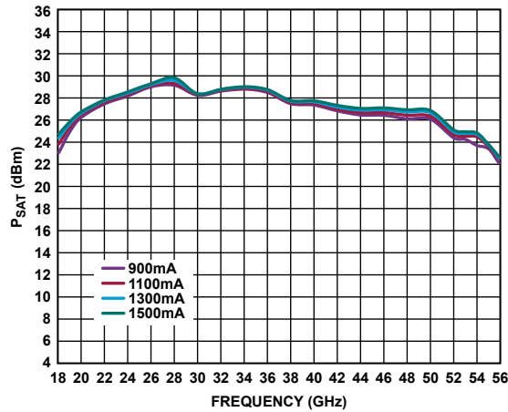
Figure 60. P_{SAT} vs. Frequency for Various Supply Currents, V_{DD} = 3\text{ V}
