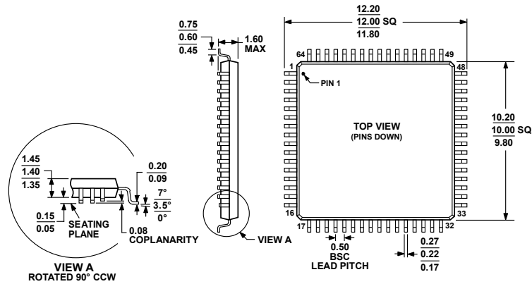
Figure 63. 64-Lead Low Profile Quad Flat Package [LQFP] (ST-64-2)
