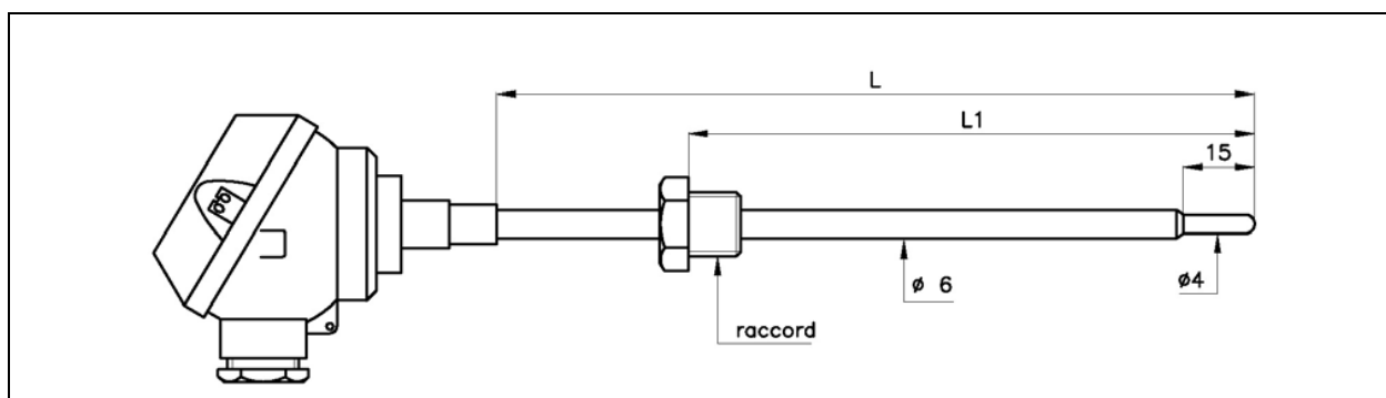
RTD SENSOR AT RESISTANCE WITH HEAD AND LINK
