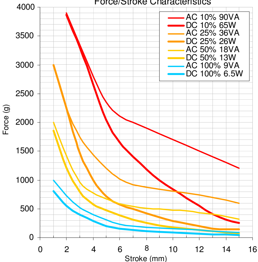
Force/Stroke Characteristics
