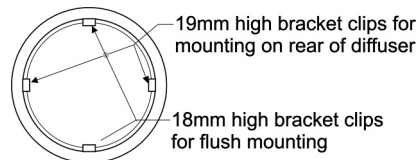
Flange Mount Bracket Detail
