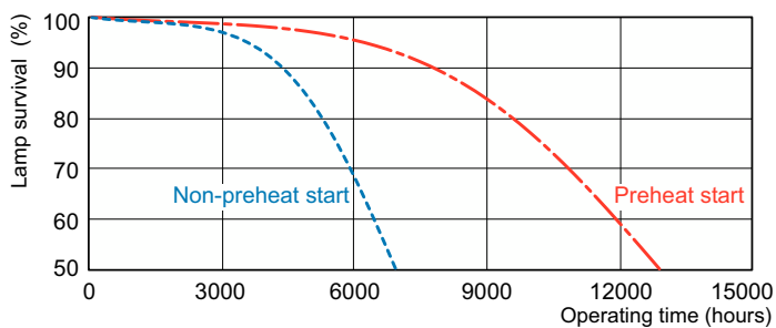
Life Expectancy Diagram - MASTER PL-C 26W/830/4P 1CT/5X10BOX
