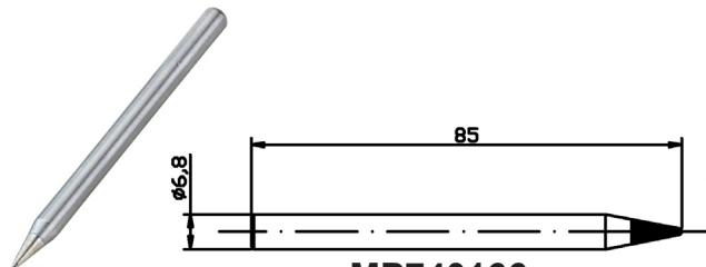
MP740166 Pointed
