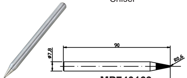
MP740169 Pointed
