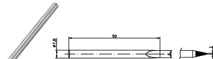
MP740170 Chisel
