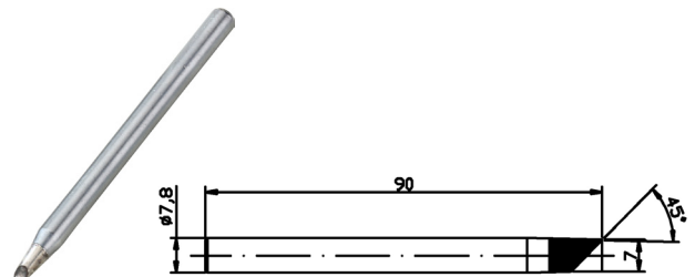
MP740171 Conical
