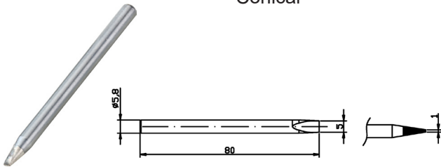
MP740164 Chisel
