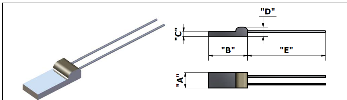
FLAT PT100Ω THERMIC ELEMENT
