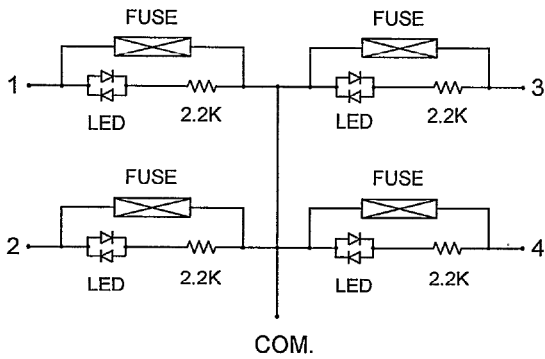
Circuit Diagram
