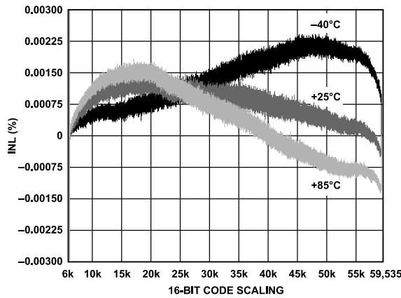
Figure 25. Normal Power Mode INL
