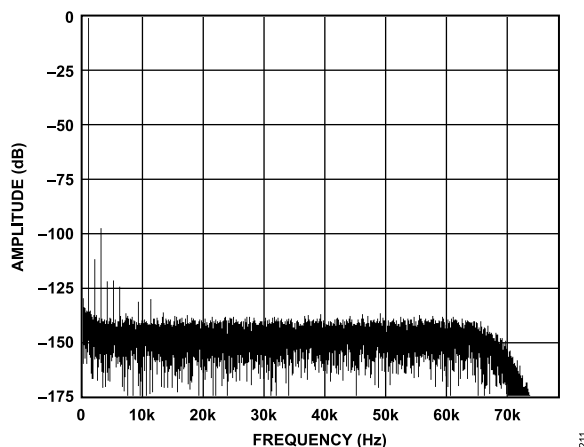
Figure 10. Low Power Mode, FFT, 1 kHz, -0.5\text{ dB} Input Tone, 128x Decimation Rate
