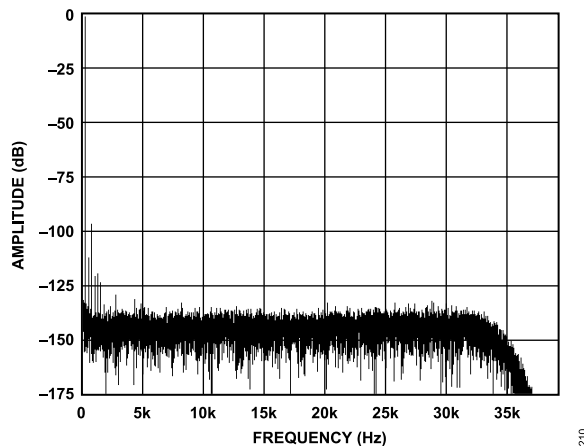
Figure 11. Low Power Mode, FFT, 1 kHz, -0.5\text{ dB} Input Tone, 256x Decimation Rate
