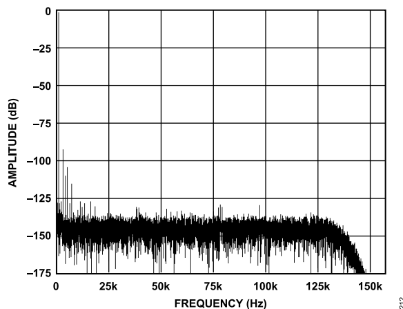
Figure 9. Low Power Mode, FFT, 1 kHz, -0.5\text{ dB} Input Tone, 64x Decimation Rate
