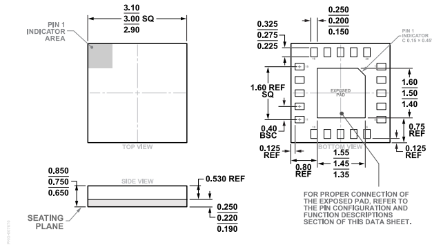
Figure 18. 20-Terminal Land Grid Array [LGA] 3 mm × 3 mm Body and 0.75 mm Package Height (CC-20-17) Dimensions Shown in Millimeters
