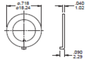
Locking ring supplied with B13,B16,B20 bushing
