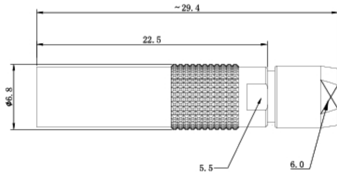
CONNECTOR SOLDER CUP VIEW
