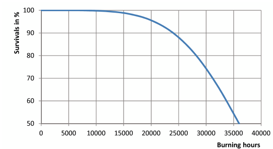
Life Expectancy Diagram - MST SON-T PIA Plus 400W E E40
