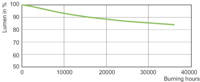
Lumen Maintenance Diagram - MST SON-T PIA Plus 400W E E40
