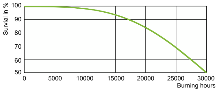
Life Expectancy Diagram - SON-T 400W E E40 1SL/12
