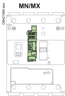
3/4 poles device in 4 poles footprint
