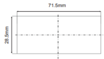
Panel cut-out
