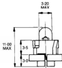
Lamp Dimensions
