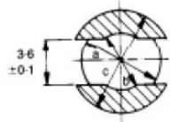
Hole Cut-out
