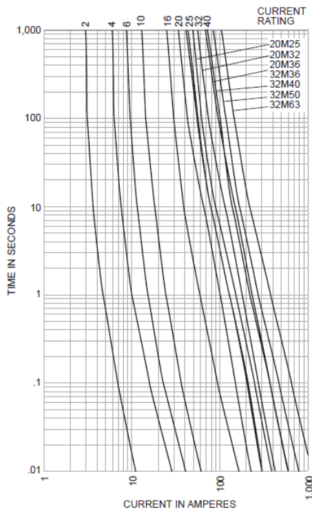
Time-Current Characteristic Curve (Full Size Curves Available)
