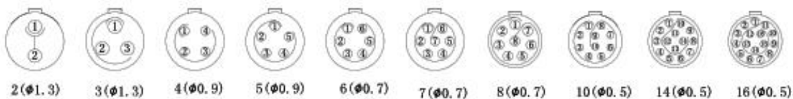
CONNECTOR SOLDER CUP VIEW
