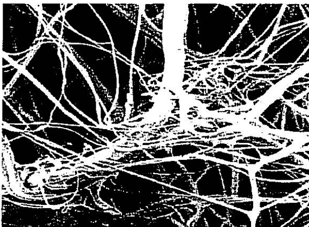
Magnified image of Acoustic Insulation showing fine PP and larger PE fibres.
