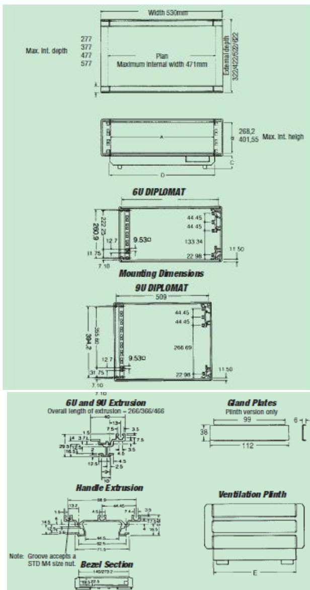
DIPLOMAT 19" Cases 6U and 9U horizontal versions
