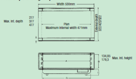
DIPLOMAT 19" Cases 3U and 4U horizontal versions
