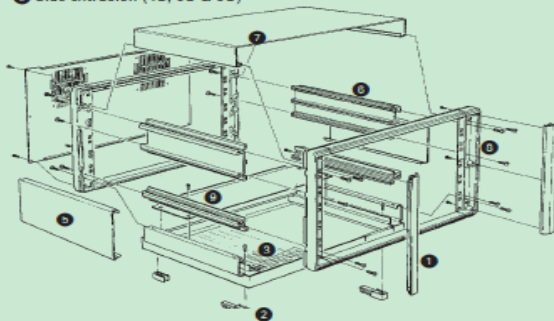
Recess trim
