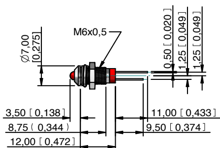
SHORT BODY PINS
