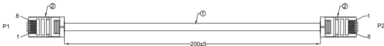
Cat6, RJ45 Plug to RJ45 Plug L=200mm(M)
