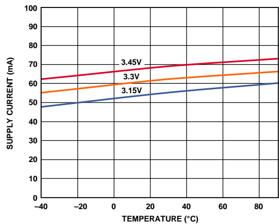
Figure 27. Supply Current vs. Supply Voltage and Temperature, 3.3 V (Using 2140 MHz Matching Components)
